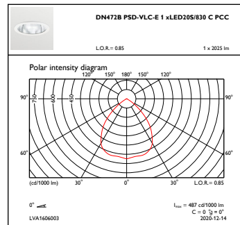
OFPC1_DN472BPSD-VLC-E1xLED20S830CPC
