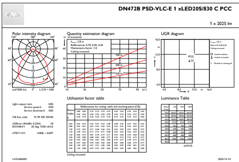
IFGU1_DN472BPSD-VLC-E1xLED20S830CPC
