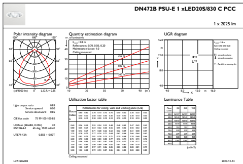
IFGU1_DN472BPSU-E1xLED20S830CPCC
