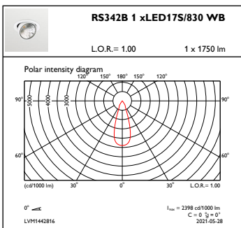
OFPC1_RS342B1xLED17S830WB
