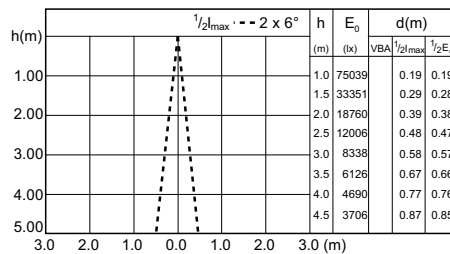
LDDBE_CDM-R-E_0003-Beam diagram
