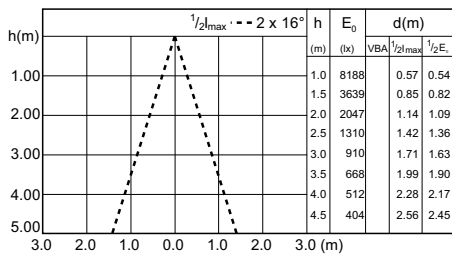
LDDBE_CDM-R-E_0001-Beam diagram
