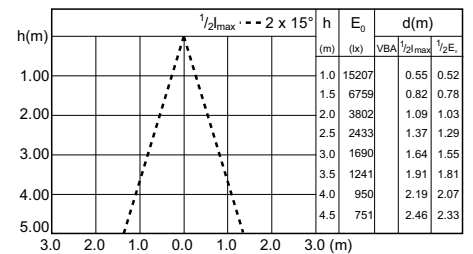
LDDBE_CDM-R-E_0004-Beam diagram
