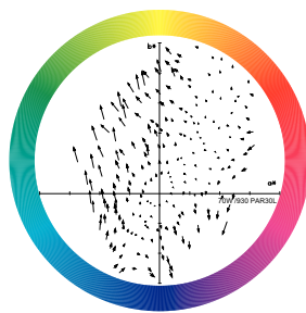
LDCR_CDM-R-E_70W_930_PAR30L-Colour rendering diagram
